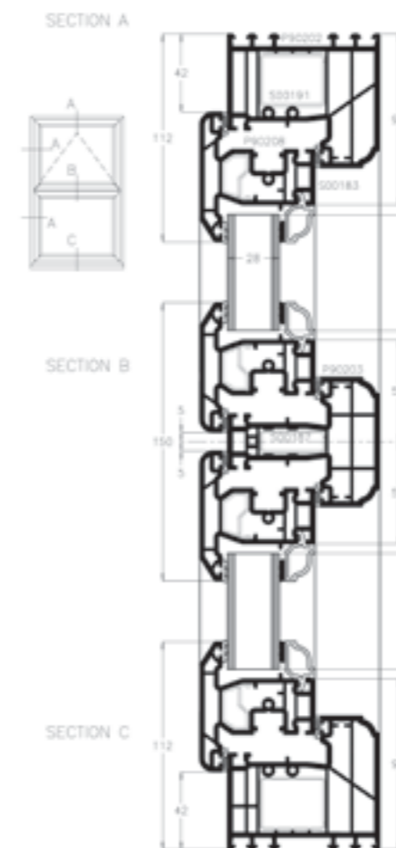
Storm 2 72mm outer frame (large)
