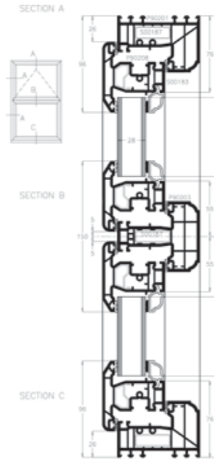
Storm 2 56mm outer frame (small)
