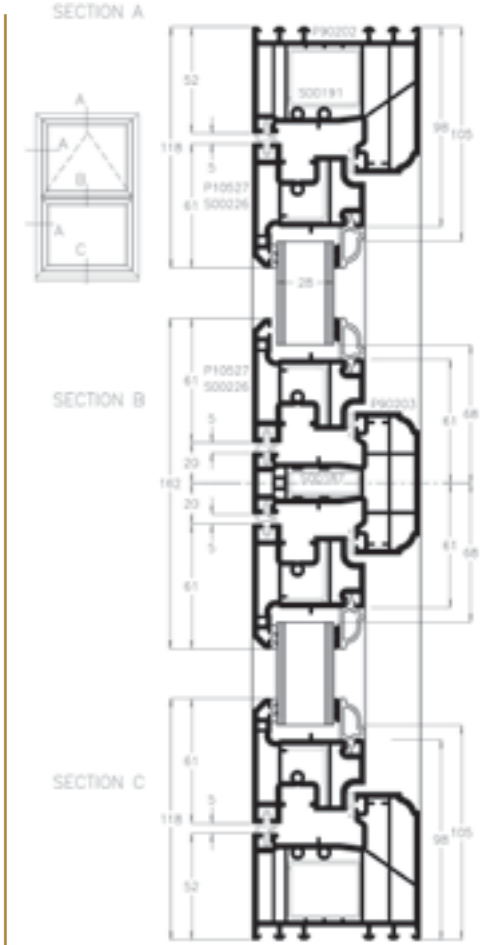
Flush 72mm outer frame (large)
